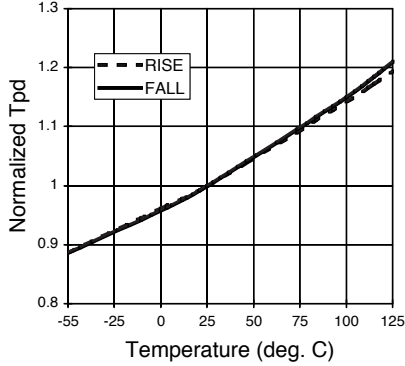
Normalized Tpd vs Temp
